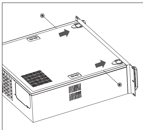
8. Assemble the Top Cover.
