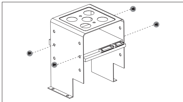
5. 6x 3.5" HDD can be installed on the HDD cages.
