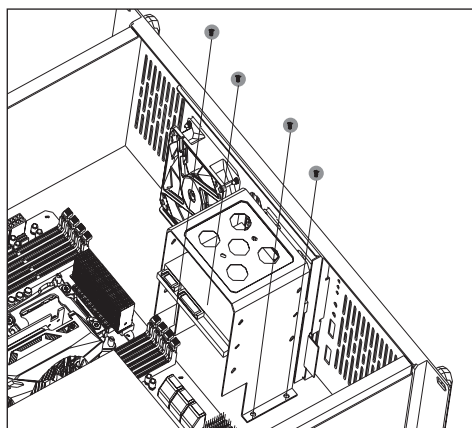
7. Install HDD cages.
